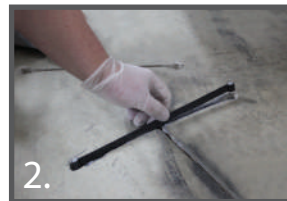
2. Press the Concrete Crack Lock® into epoxy
